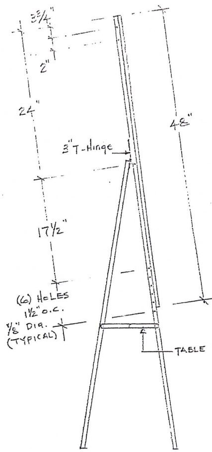
SIDE VIEW SCALE 3/4"=1'-0"
